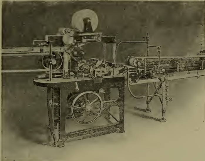
Floor space of machine, 3 feet by 18 feet; weight, 2,800 pounds. Speed of delivery guaranteed. Formerly manufactured by Thos. F. Condon & Co.
